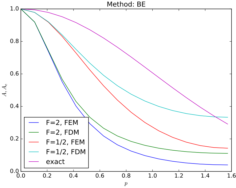
Fig. 7.2 Comparison of coarse-mesh amplification factors for Backward Euler discretization of a 1D diffusion equation.
