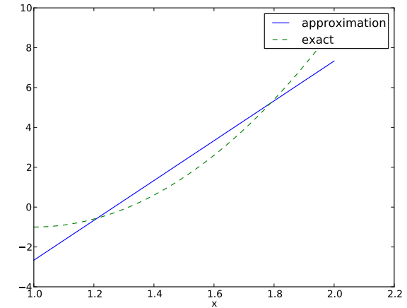
Fig. 3.2 Best approximation of a parabola by a straight line.
