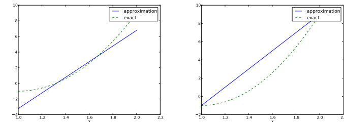
Fig. 3.9 Approximation of a parabola by linear functions computed by two interpolation points: 4/3 and 5/3 (left) versus 1 and 2 (right).
