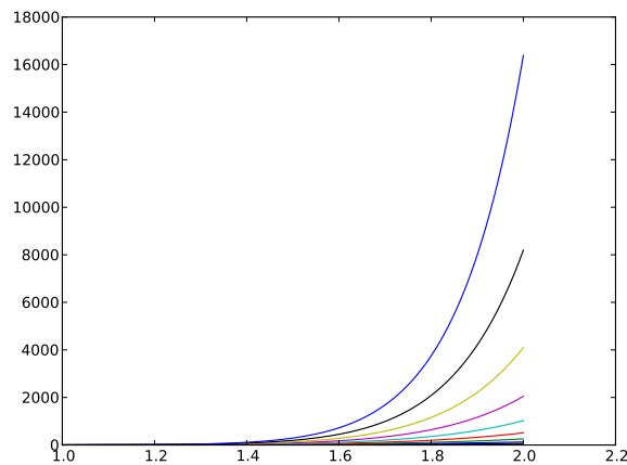
Fig. 3.6 The 15 first basis functions x^i , i = 0, \dots, 14 .
